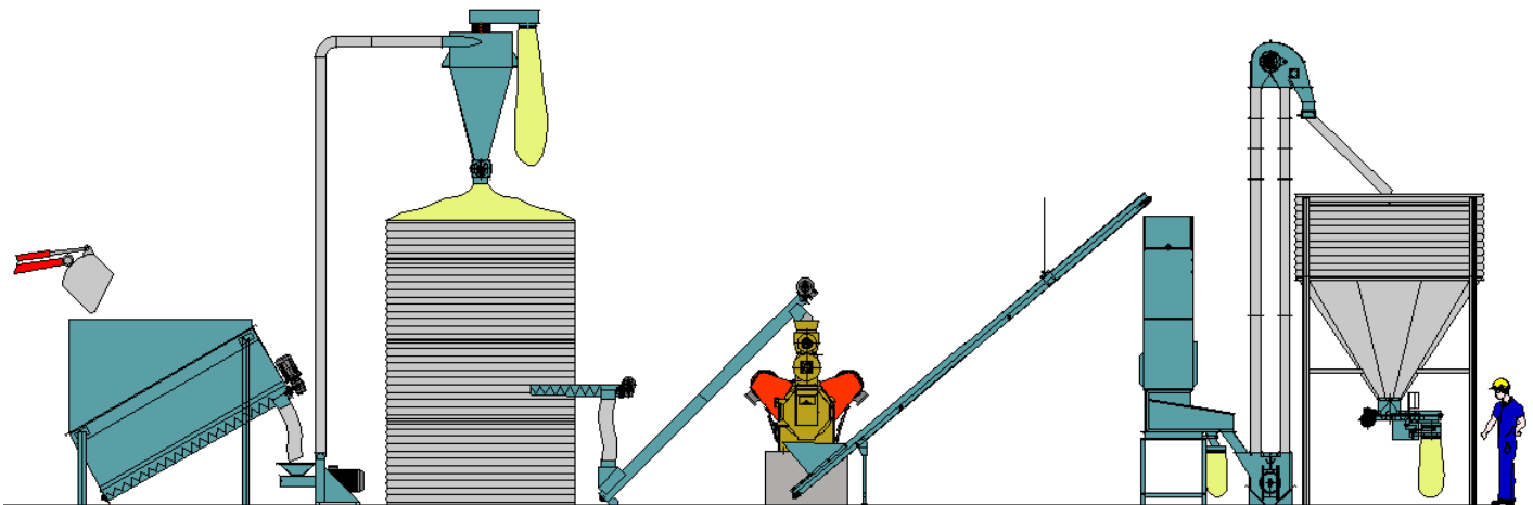
MILLING LINE - PELLETISING OF SAWDUST AND WOOD CHIPS
