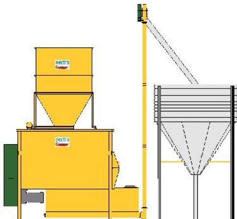
BMH assembly for electronic weighing
